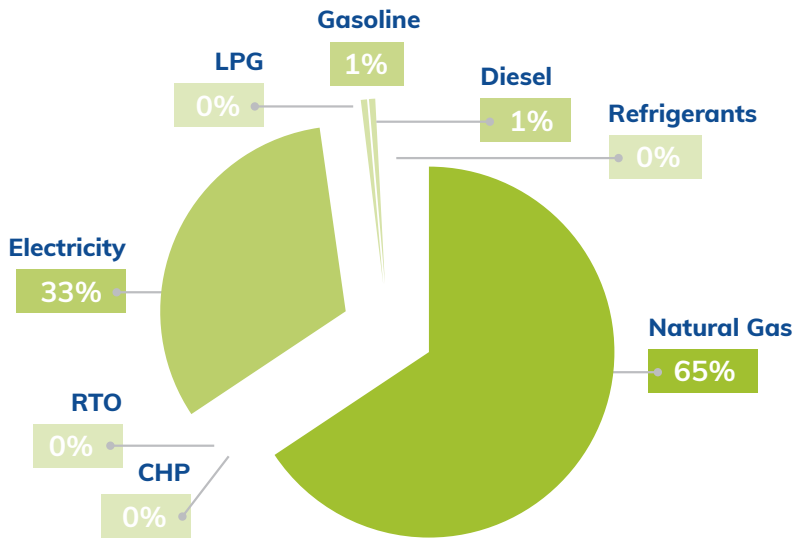
Share of emissions, by emission category (in %)
