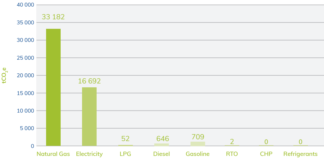
Total direct emissions, by emission category
