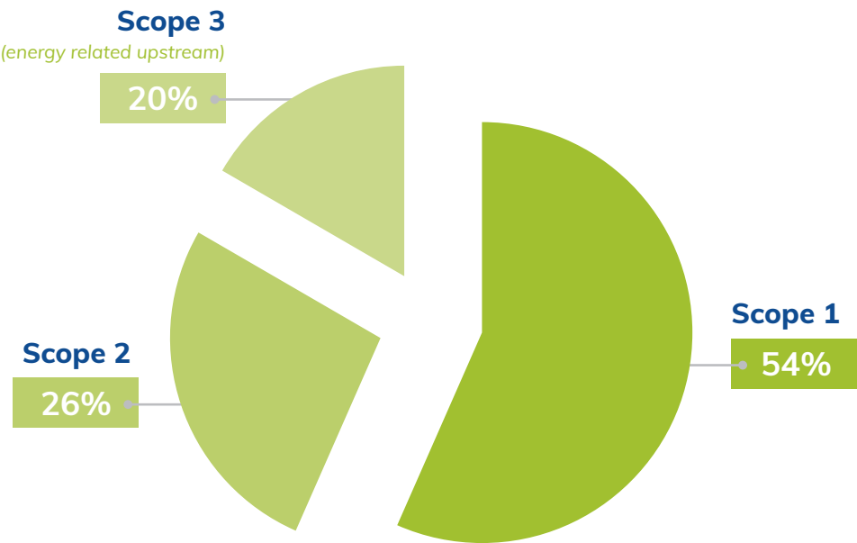
Share of emissions by scope (in %)
